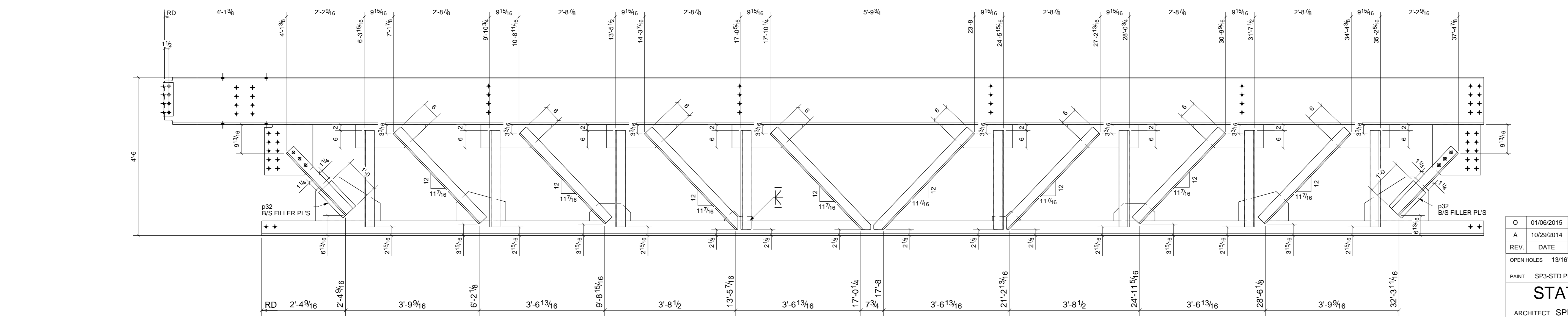
ONE - TRUSS_T-1a - 121B1
